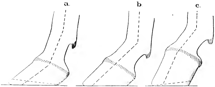
FIG. 6.—Limbs and hoofs in profile: a , Side view of foot with the foot-axis broken backward as a result of too long a toe. The amount of horn to be removed from the toe in order to straighten the foot-axis is denoted by a dotted line; b , side view of a properly balanced foot, with a straight foot-axis of desirable slant; c , side view of stumpy foot with foot-axis broken forward as a result of overgrowth of the quarters. The amount of horn to be removed in order to straighten the foot-axis is shown by a dotted line.
